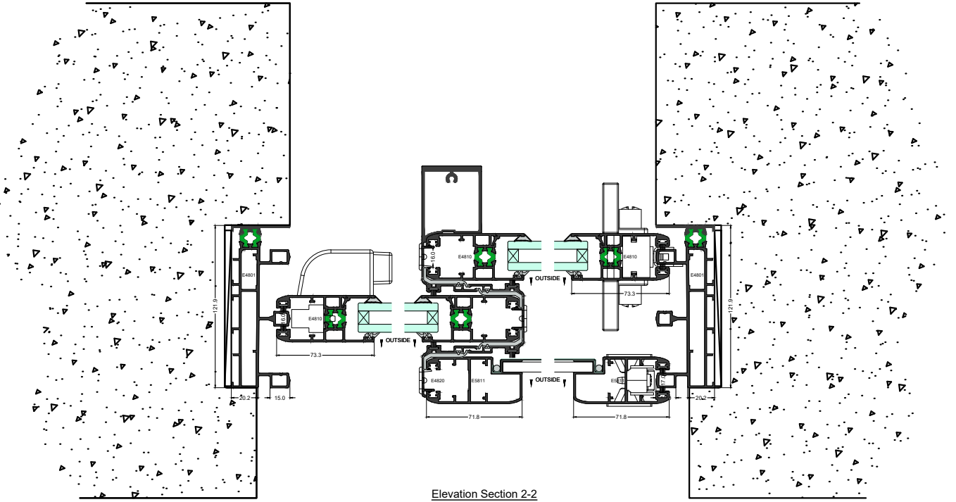
Elevation Section 2-2
