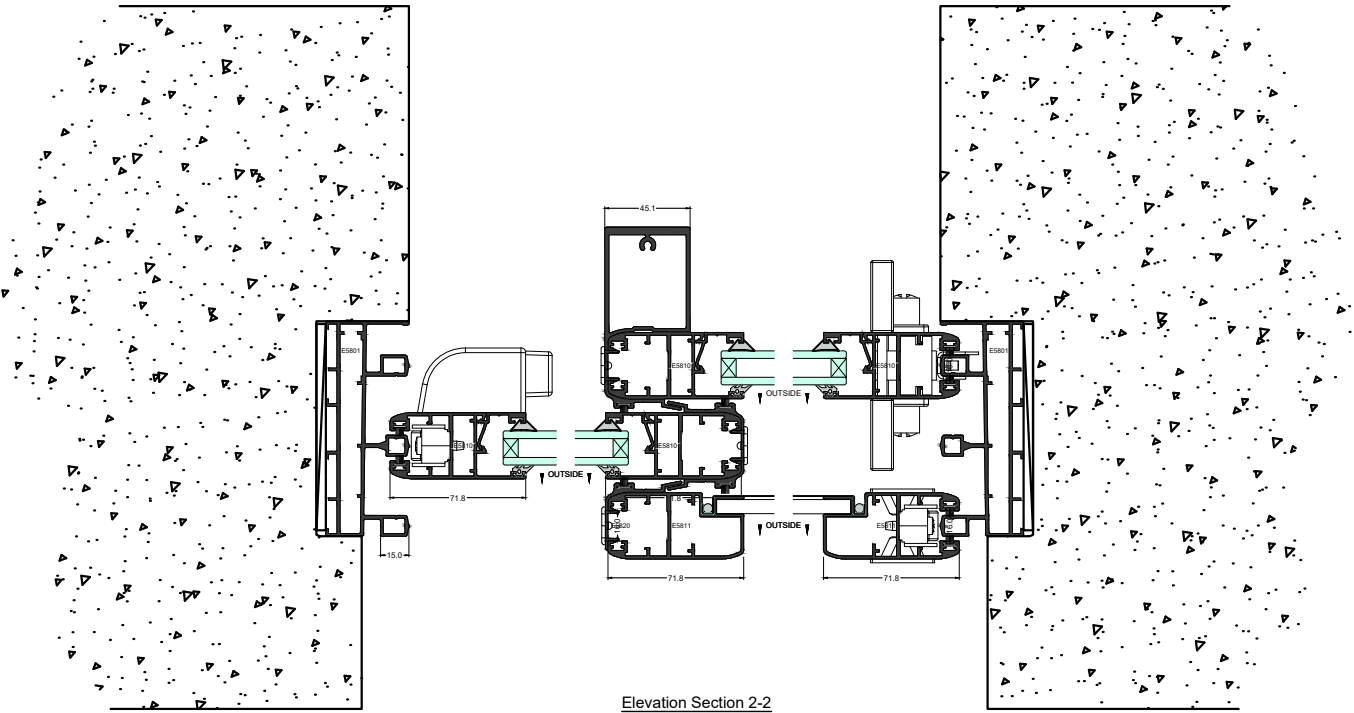
Elevation Section 2-2
