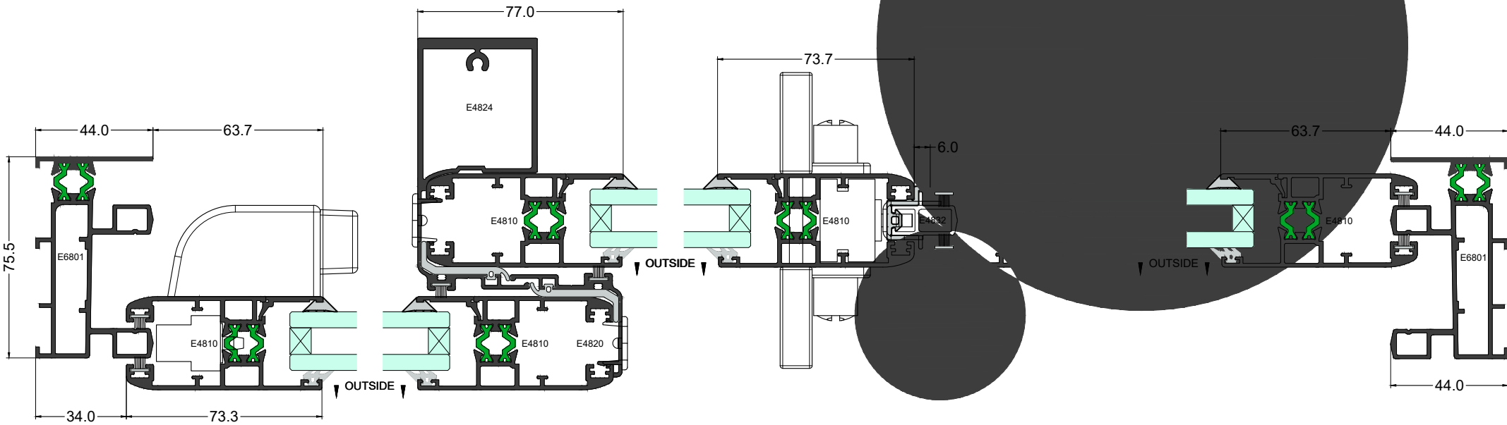
Plan Section 7-7
