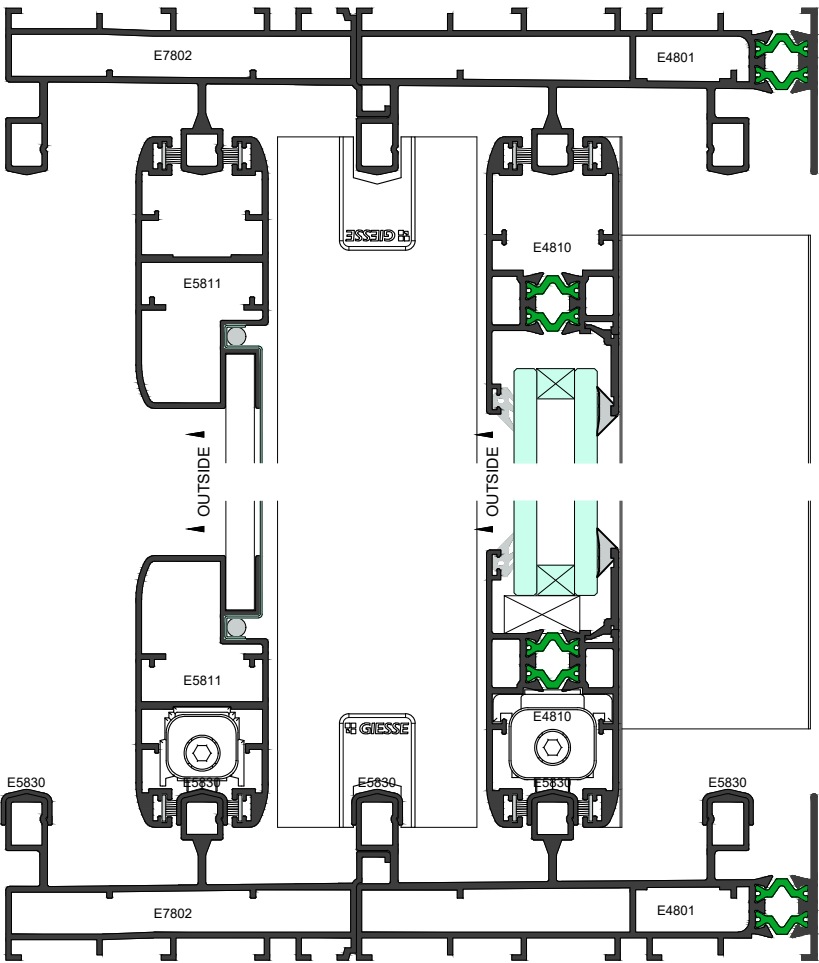
Elevation Section 12-12
