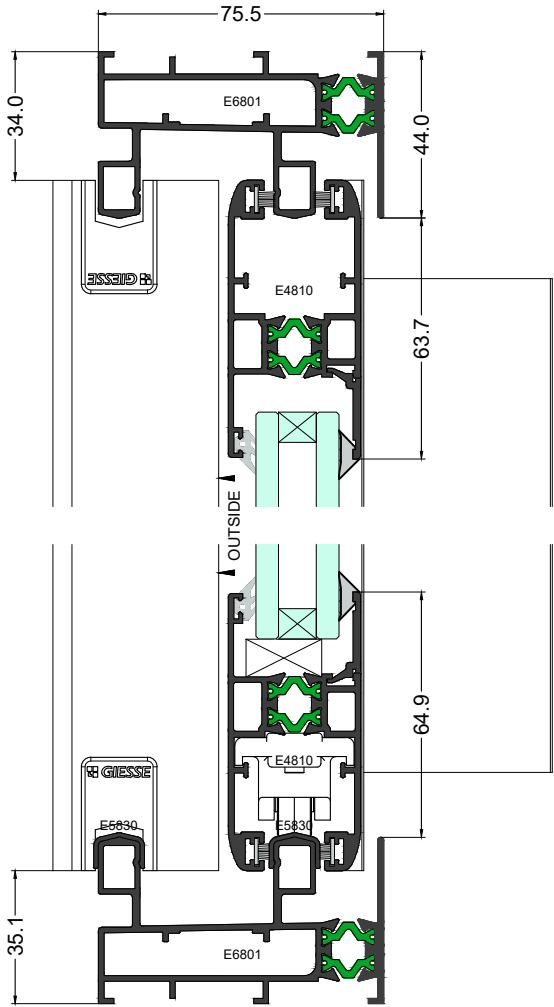
Elevation Section 6-6
