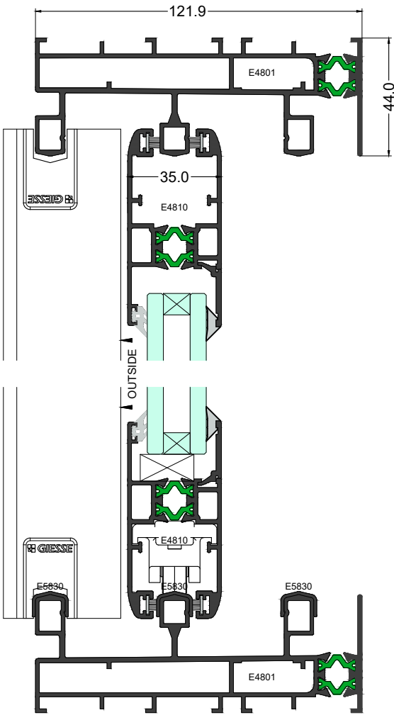
Elevation Section 8-8
