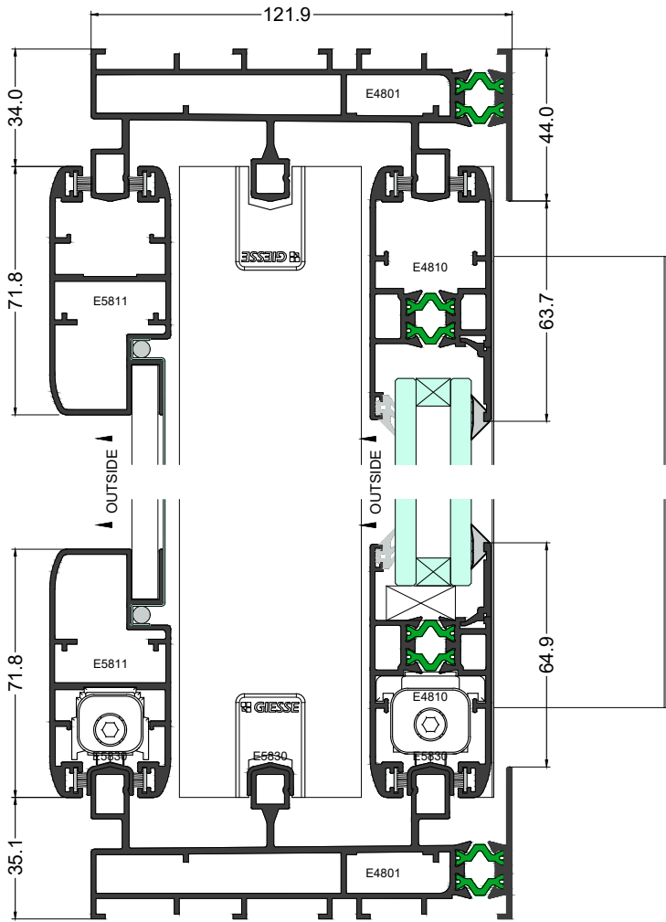
Elevation Section 2-2
