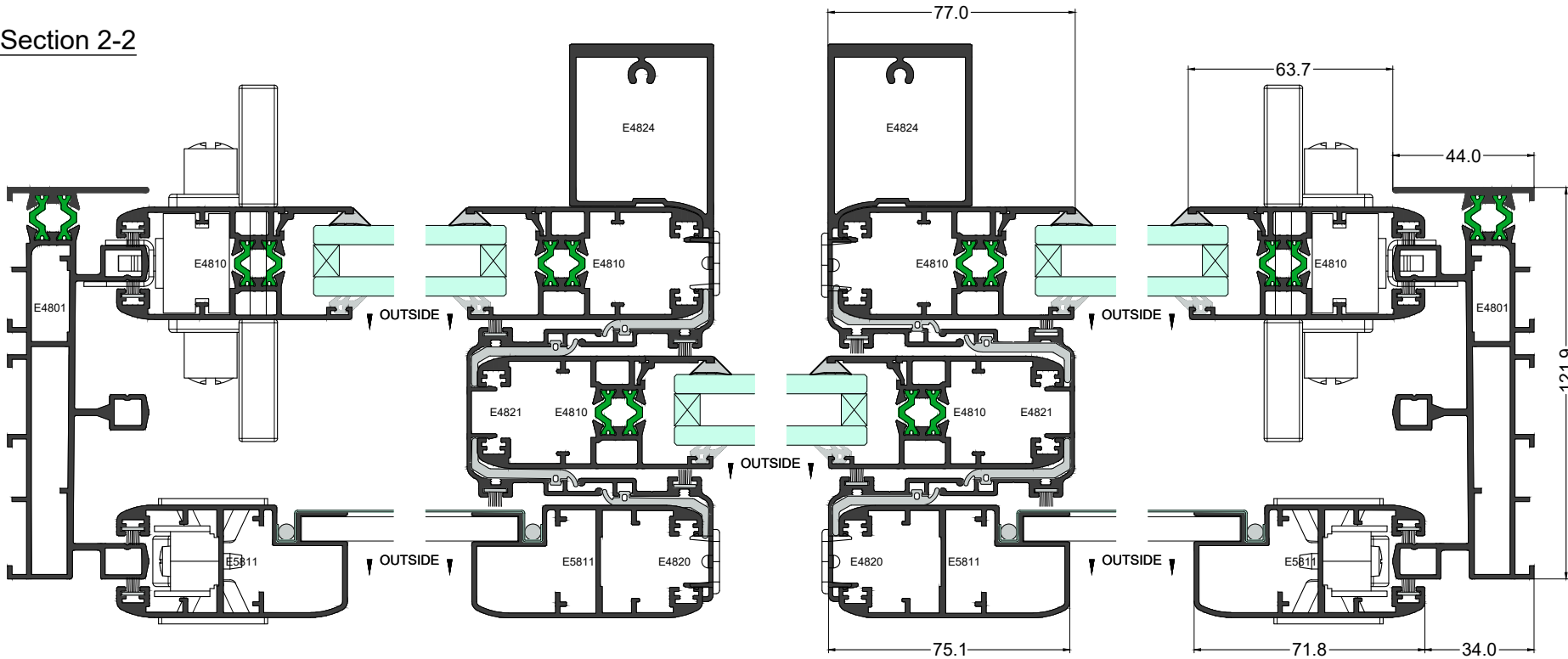
Plan Section 9-9
