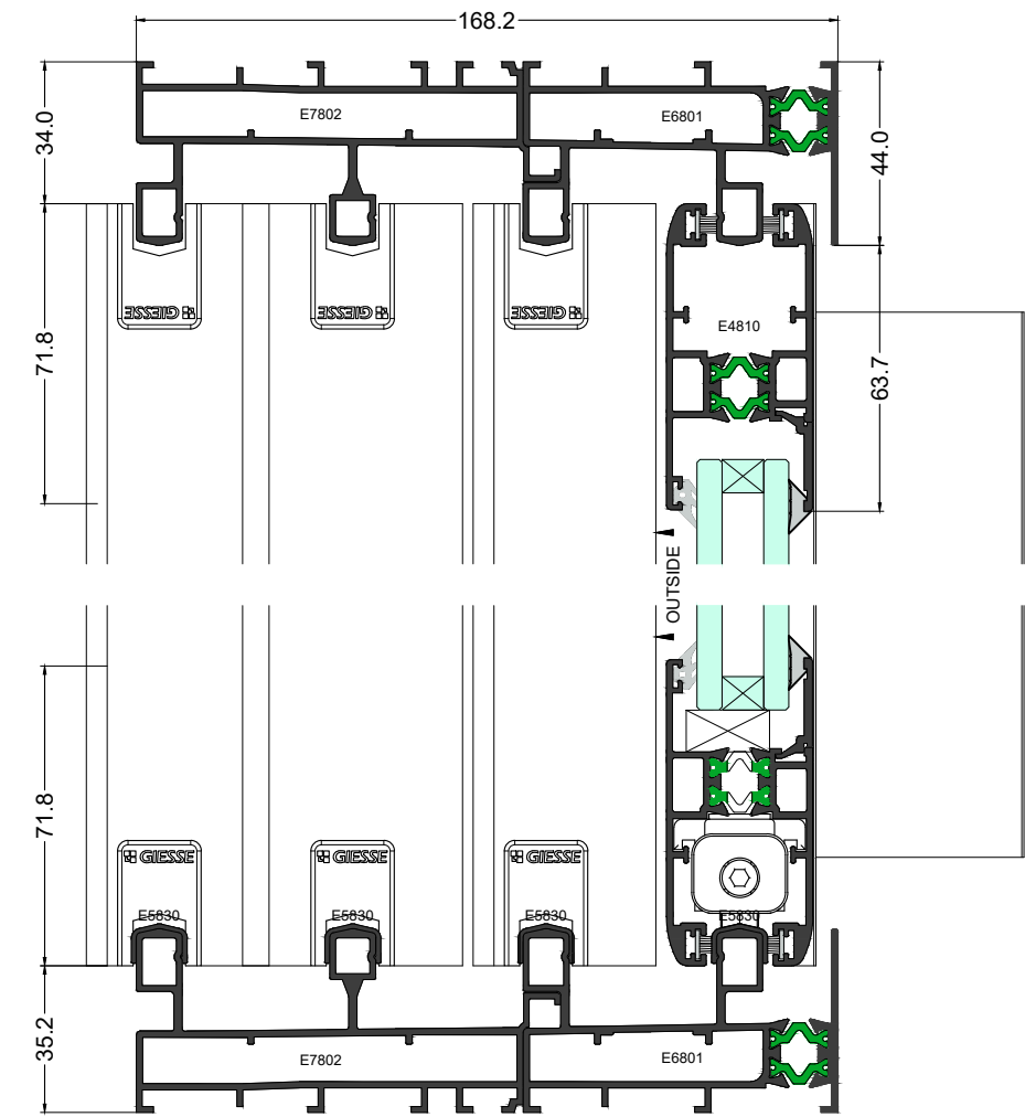
Elevation Section 16-16
