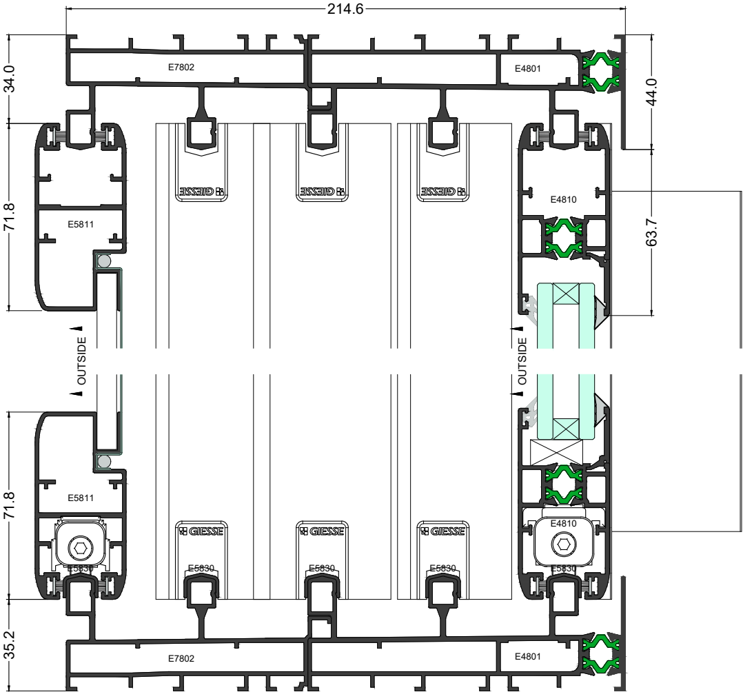
Elevation Section 13-13
