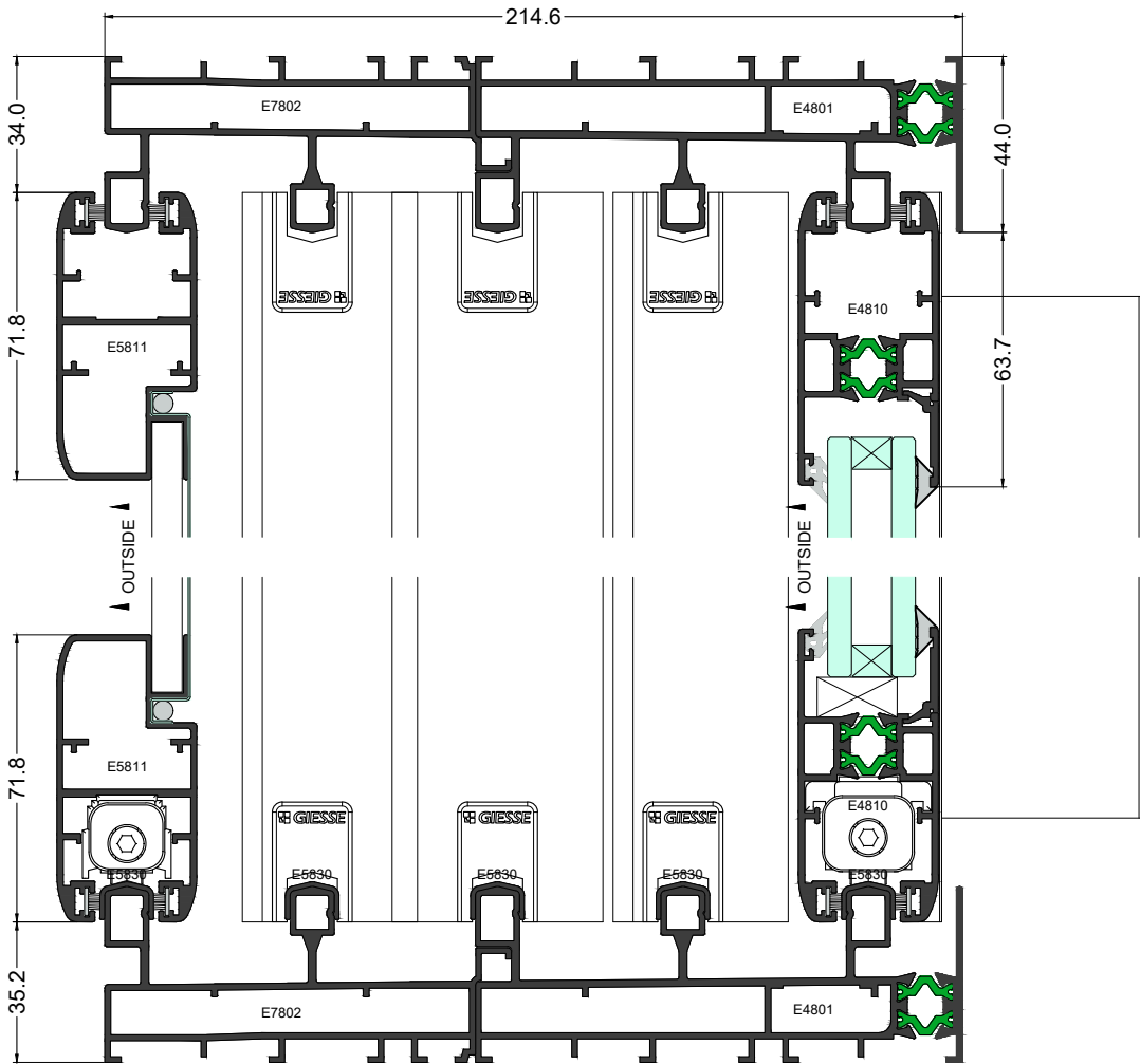
Elevation Section 13-13
