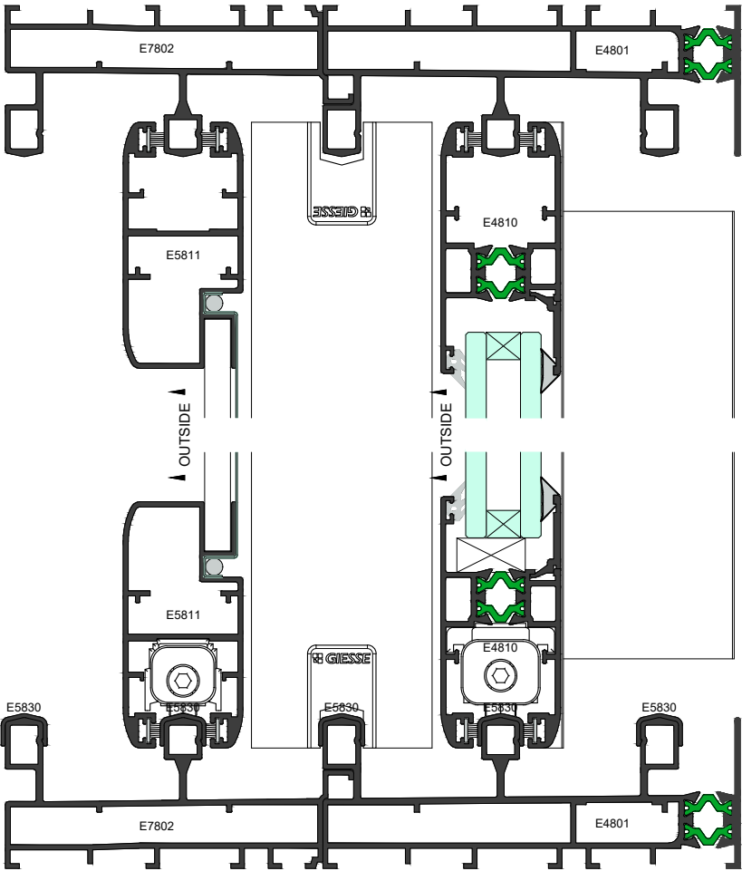
Elevation Section 12-12
