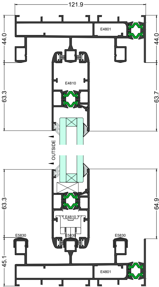
Elevation Section 1-1
