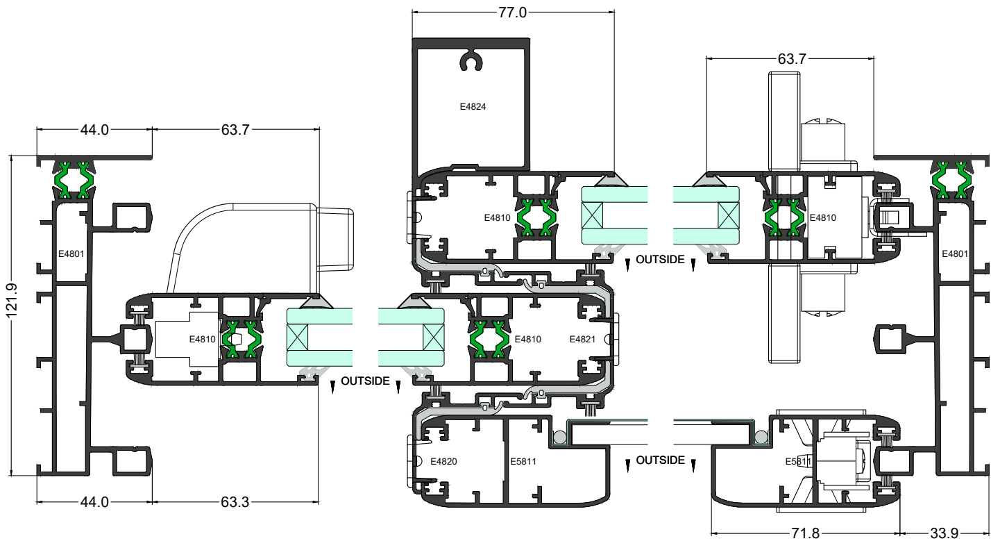
Plan Section 3-3
