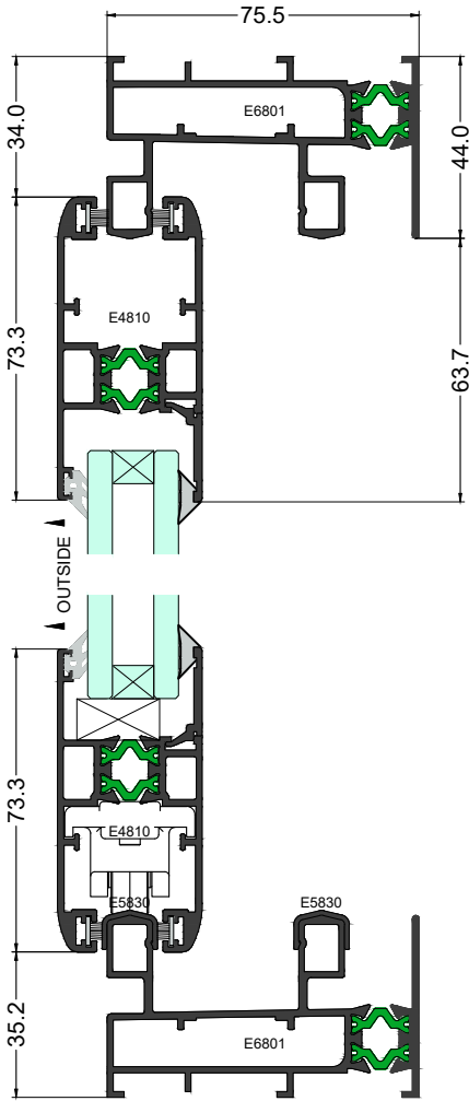
Elevation Section 4-4
