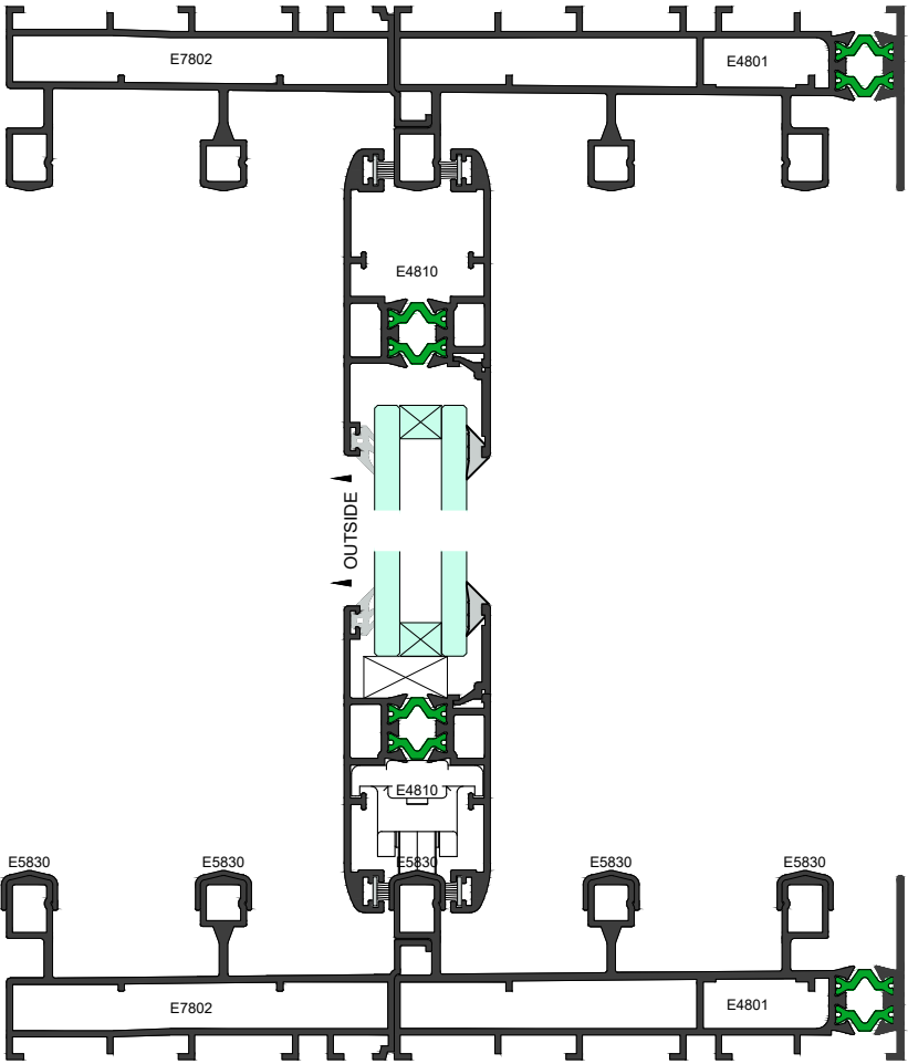
Elevation Section 11-11
