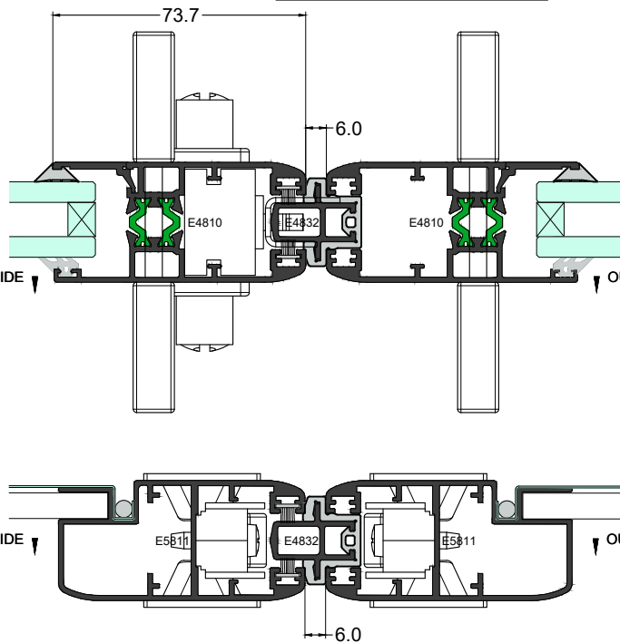
Plan Section 10-10
