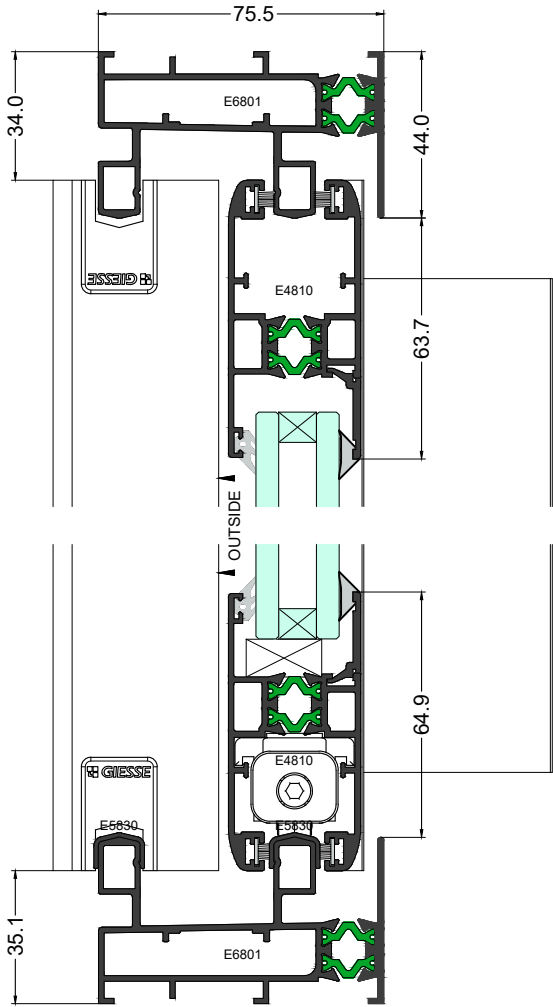
Elevation Section 5-5
