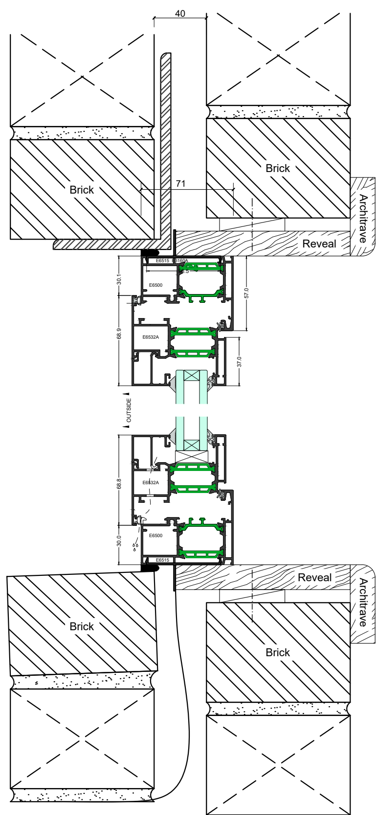
Elevation Section 1-1
