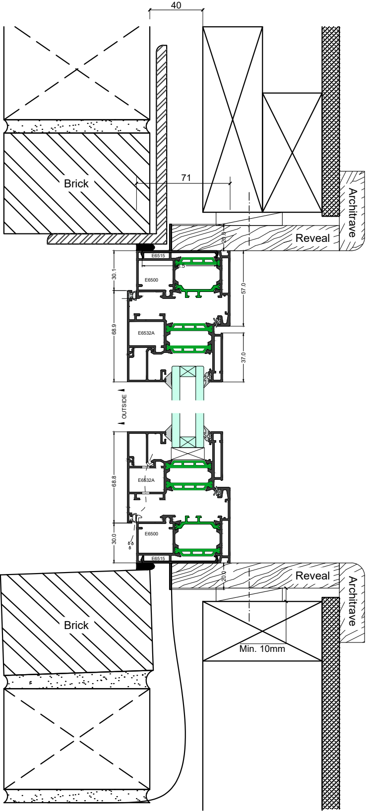
Elevation Section 1-1
