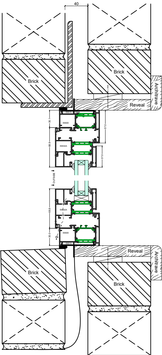
Elevation Section 1-1
