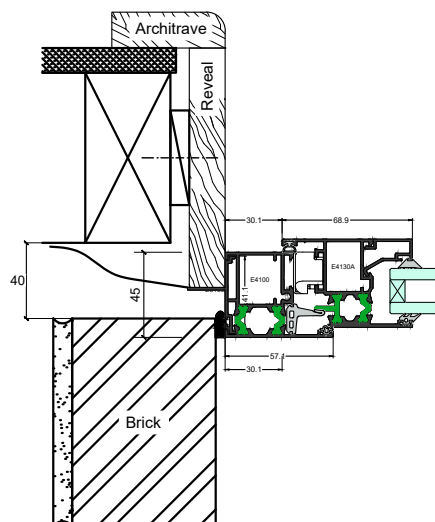
Elevation Section 1-1
