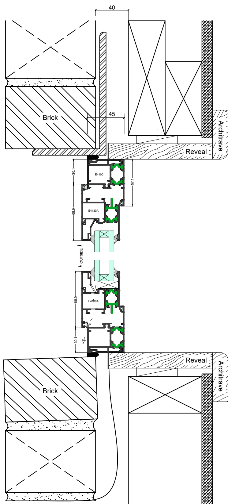
Elevation Section 1-1
