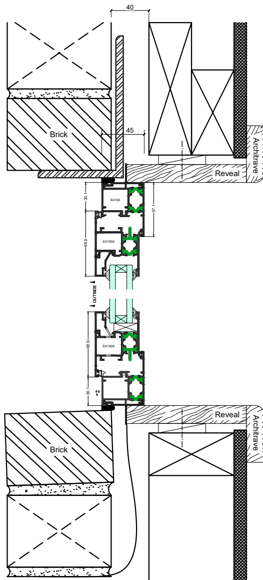
Elevation Section 1-1
