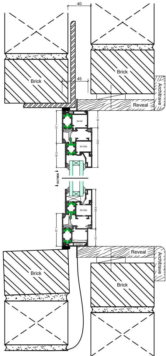
Elevation Section 1-1
