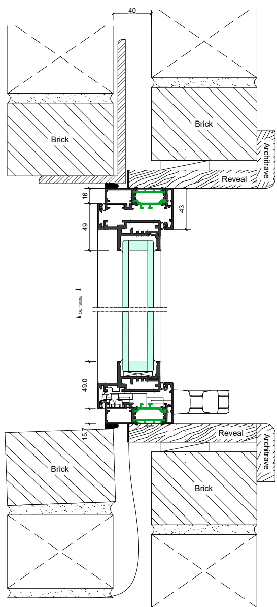
Elevation Section 1-1
