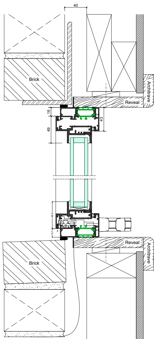
Elevation Section 1-1
