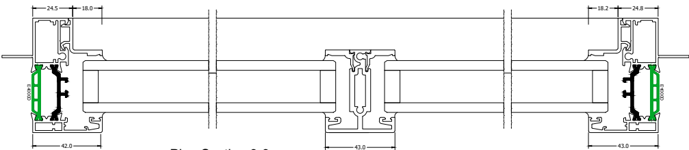
Plan Section 3-3
