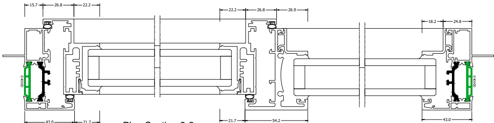
Plan Section 2-2
