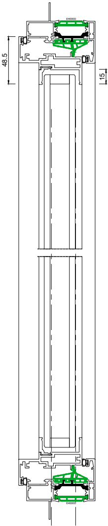
Elevation Section 2-2
