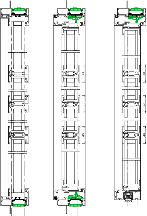
Elevation Section 5-5 Elevation Section 2-2 Elevation Section 1-1
