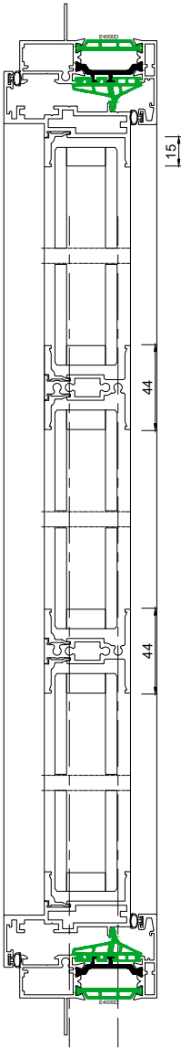
Elevation Section 2-2
