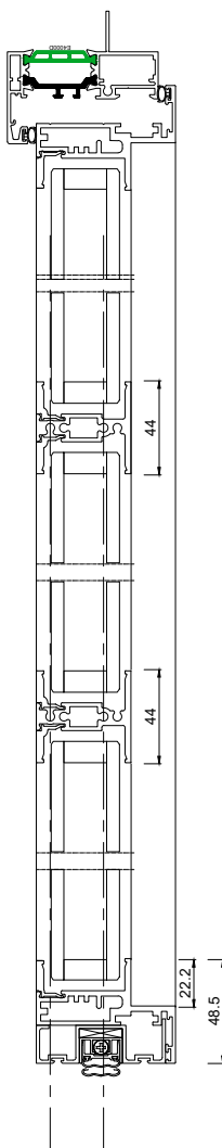
Elevation Section 1-1
