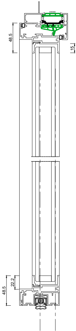
Elevation Section 1-1
