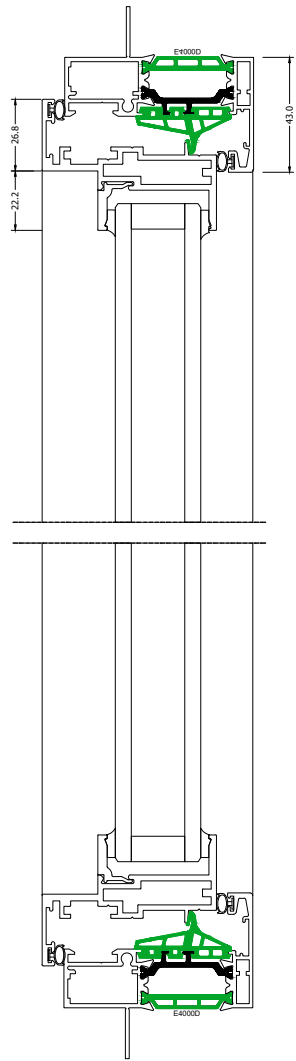
Elevation Section 1-1
