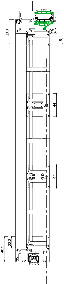
Elevation Section 1-1
