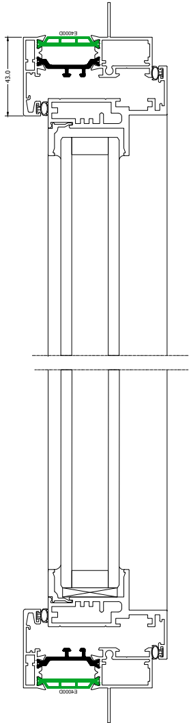
Elevation Section 1-1 Elevation Section 3-3
