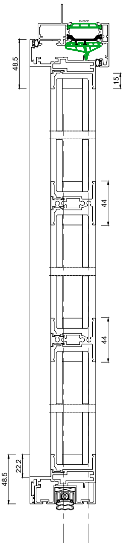
Elevation Section 1-1
