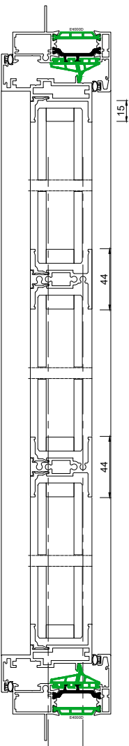
Elevation Section 2-2
