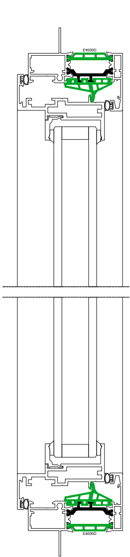
Elevation Section 1-1 Elevation Section 3-3
