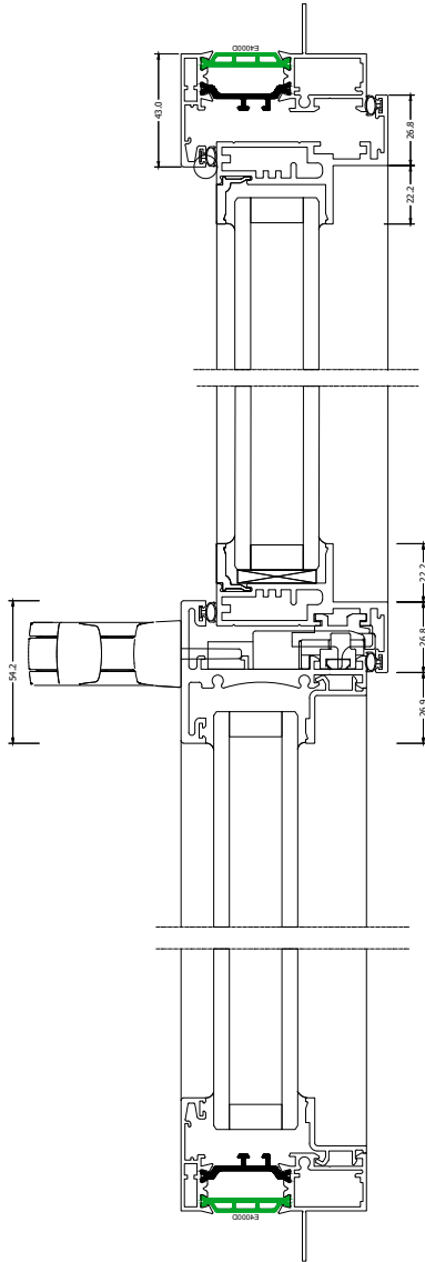
Elevation Section 1-1
