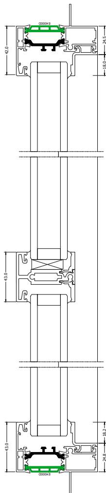
Elevation Section 1-1
