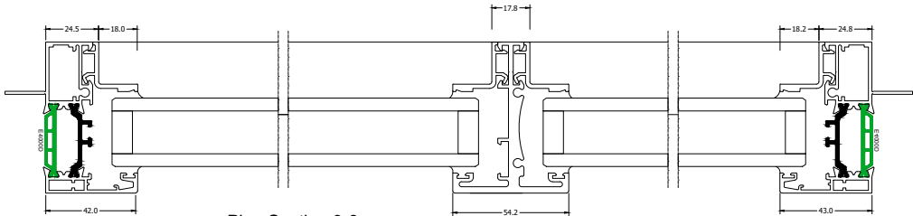
Plan Section 3-3
