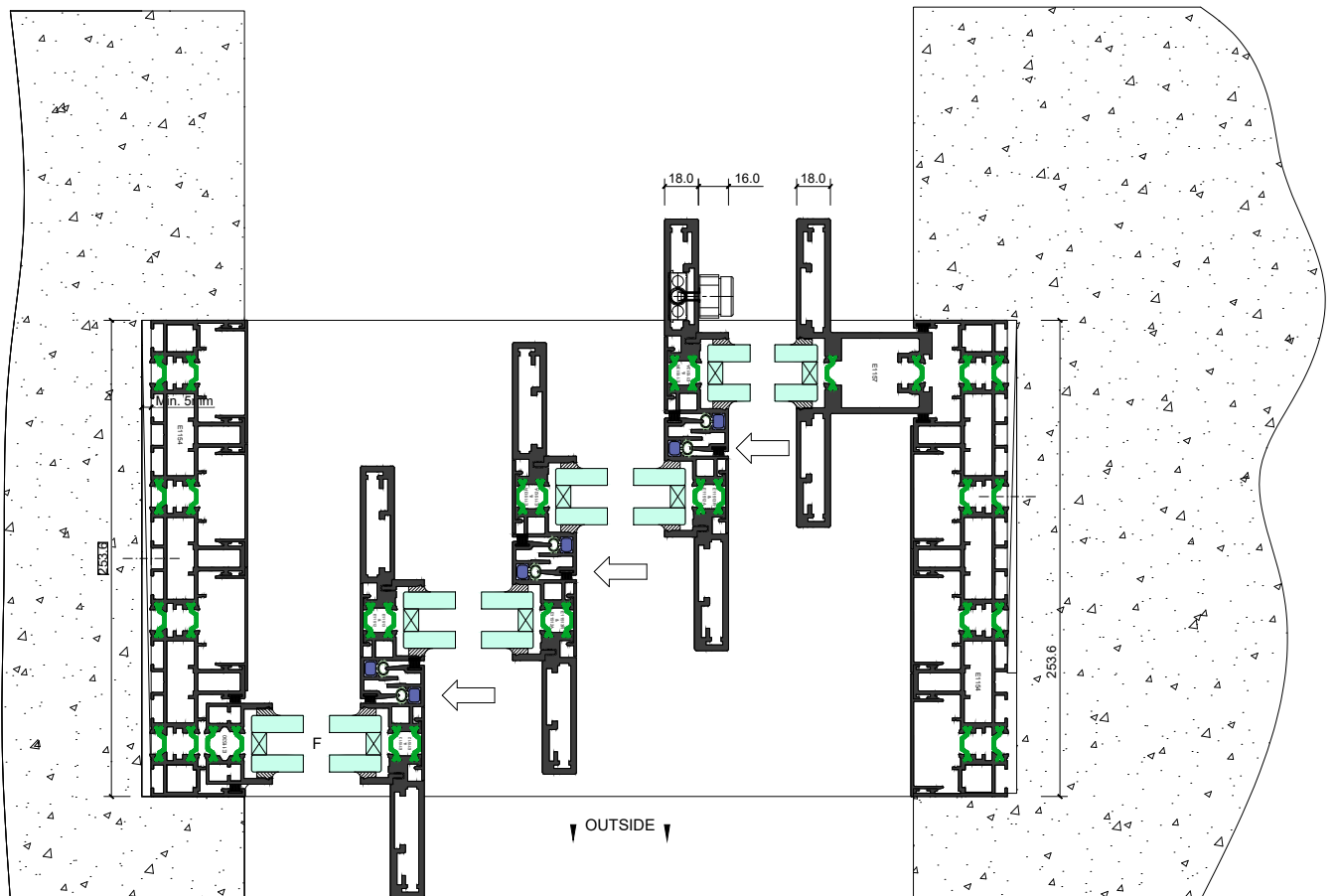
Plan Section 1-1
