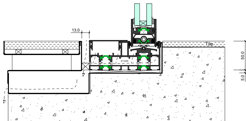
(Stainless Steel Slot Drain Option)
