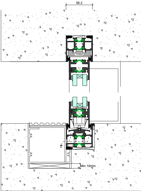
Section 2-2
