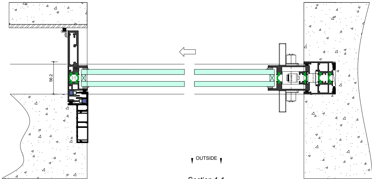
Section 1-1
